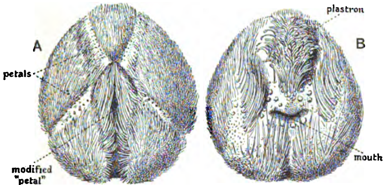
FIG. 245.— Echinocardium cordatum . A, aboral view; B, oral view. \times 1 .
